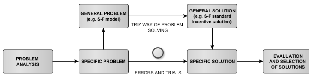
Fig. 1. A TRIZ model of problems solving with an example of the use of SU-FIELD models
